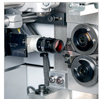
▲ WAFIOS Vision System (WVS)
