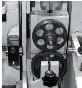
▲ Measuring wheel
