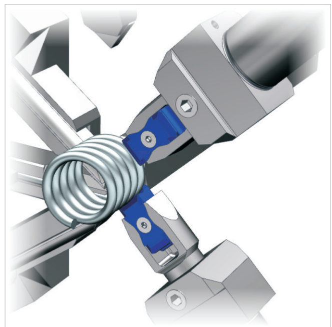
▲ Holder with coiling insert - example
